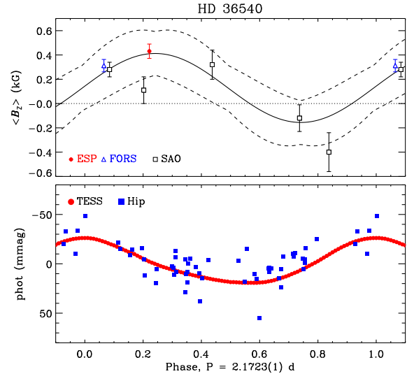
Figure C7. Top : \langle B_z \rangle measurements for HD 36540, obtained from Romanyuk et al. (2017b), Bagnulo et al. (2015a), and ESPaDONs, folded with the rotation period. Solid/dashed curves show first-order harmonic fit and uncertainty. Bottom : Hipparcos and TESS light curves folded with the rotation period. Larger points indicate phase-binned data.
