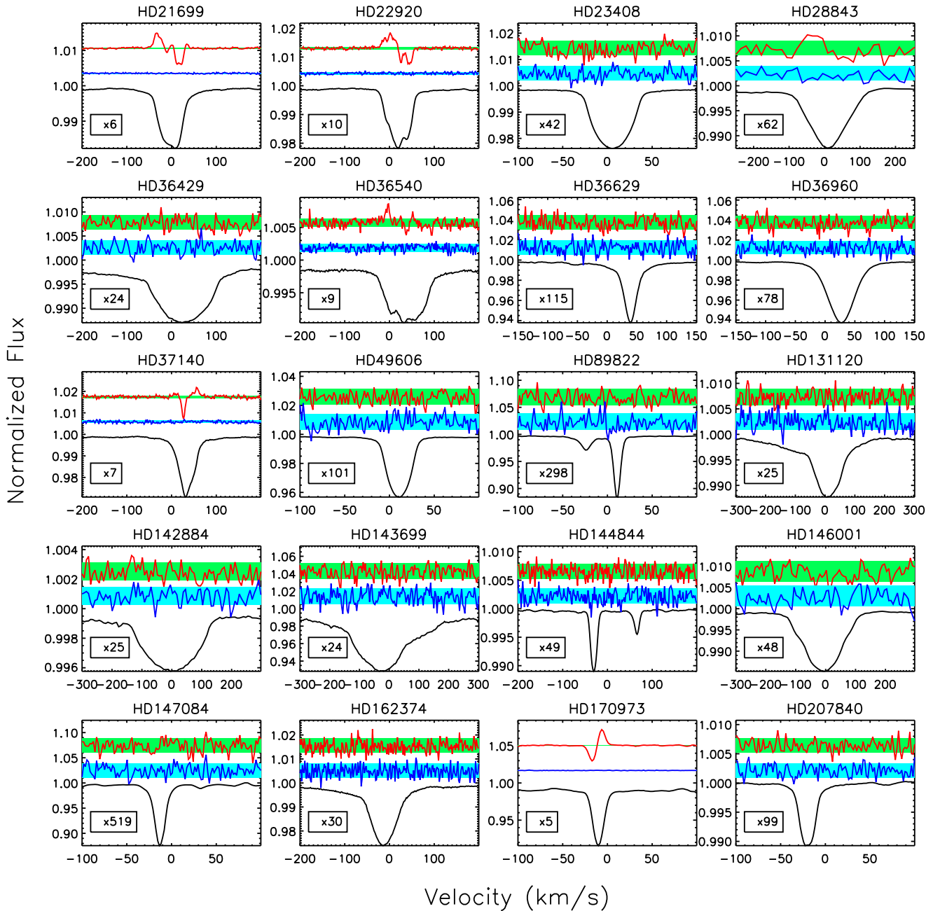
Figure C1. LSD profiles extracted from ESPaDOnS and Narval observations. Each panel shows Stokes I (black, bottom), N (blue, middle), Stokes V (red, top). Blue and green shaded regions show the mean error bars for N and Stokes V , respectively. Box gives the amplification factor for N and Stokes V .
