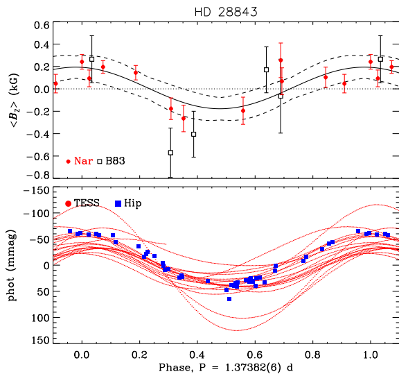
Figure C4. Top: \langle B_z \rangle measurements for HD 28843, obtained from Borra et al. (1983) and Narval, folded with the rotation period. Solid/dashed curves show first-order harmonic fit and uncertainty. Bottom: Hipparcos and TESS light curves folded with the rotation period.
