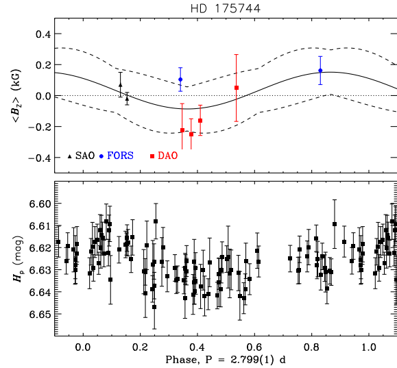
Figure C30. Top : \langle B_z \rangle measurements of HD 175744 folded with the rotation period inferred from Hipparcos photometry ( Bottom ). The harmonic fit to \langle B_z \rangle is performed to the combined magnetic dataset.
